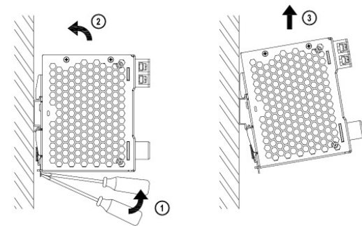
Fig. 2.2 Dismounting
