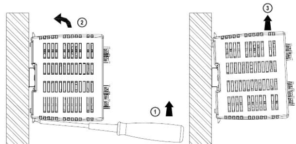
Fig. 2.2 Dismounting
